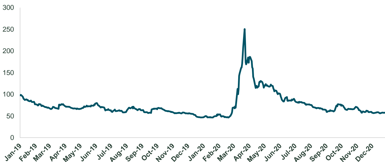
Figure 1. 5 Year iTraxx Spreads, 2 January 2019 to 31 December 2020
